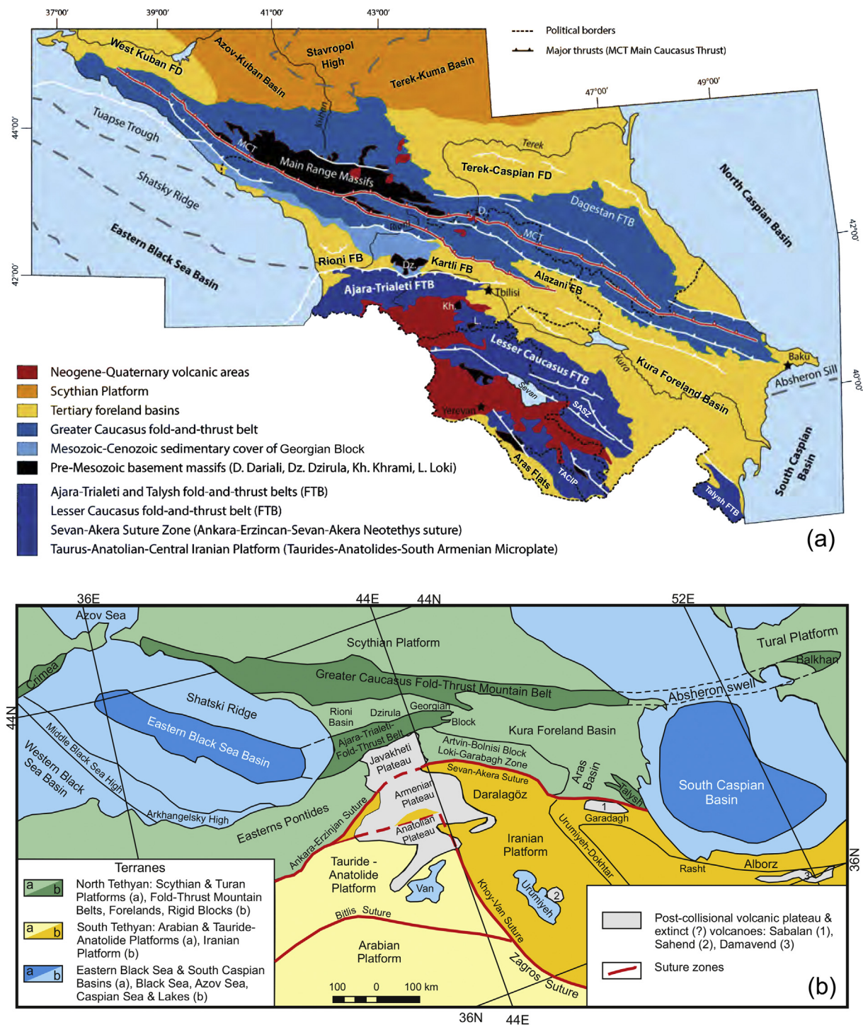
Fig. 2. (a) Main tectonic units of the Caucasus. SASZ: the Sevan-Akera Suture Zone; TACIP: the Taurus-Anatolian-Central Iranian Platform; FD: foredeep; MCT: the Main Caucasus Thrust; FTB: fold-and-thrust belt. (b) Correlation map of the main tectonic units of the Caucasus and adjacent areas (modified after Adamia et al., 2011 ).
