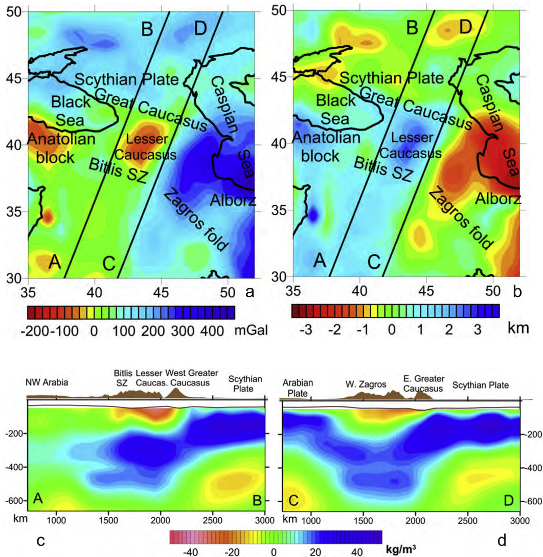
Fig. 8. Residual mantle gravity anomalies (a) and residual topography (b) induced by density variations in the upper mantle beneath the Caucasus and the surrounding region (Kaban et al., 2016, 2018). Black lines show the positions of two profiles illustrating the density model: profile AB (c) and profile CD (d).
